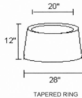
TAPERED RING
